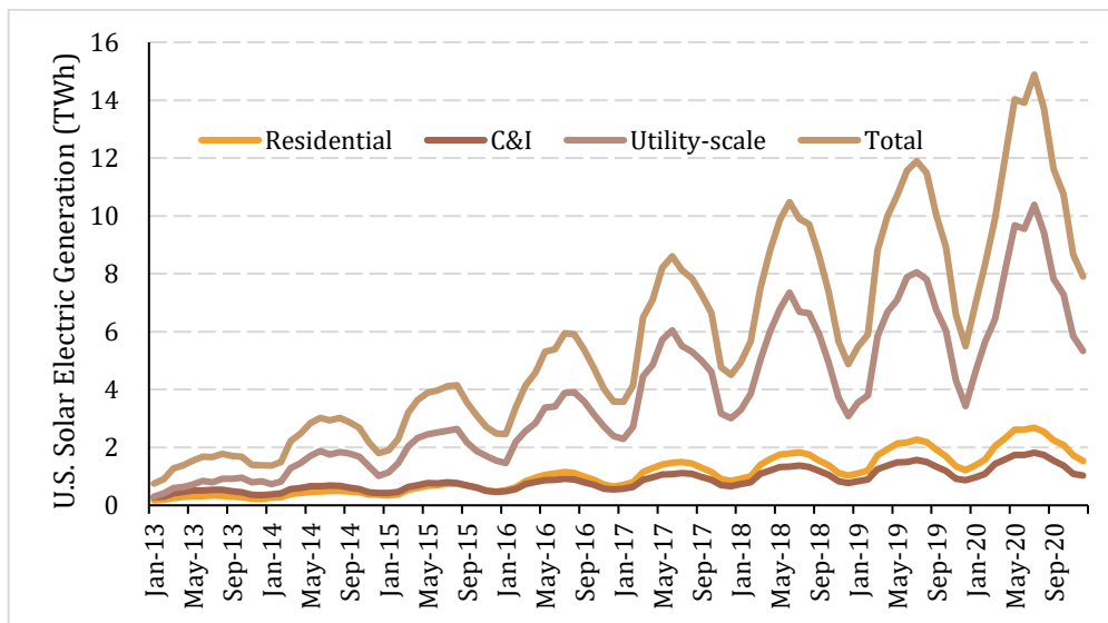
Figure 19. U.S. monthly solar production shows strong seasonal dependency
